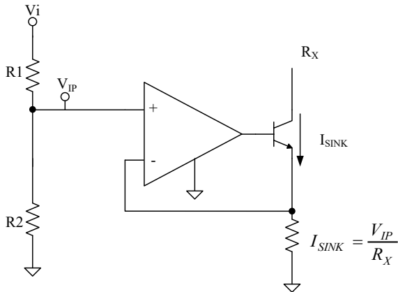
Current Sink
