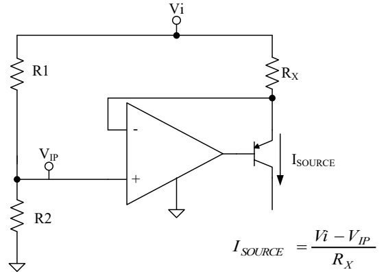
Current Source
