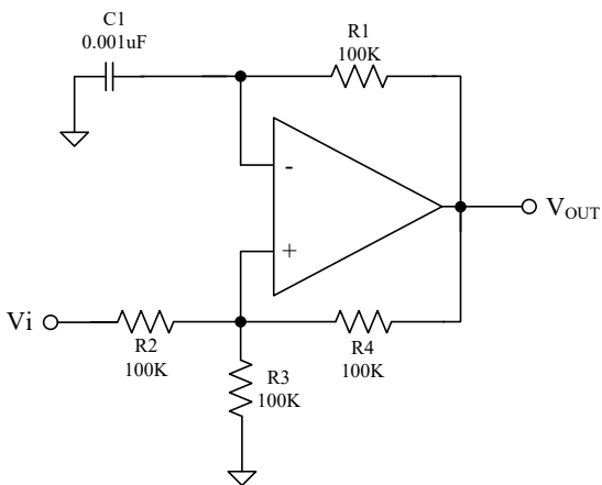
Squarwave Oscillator
