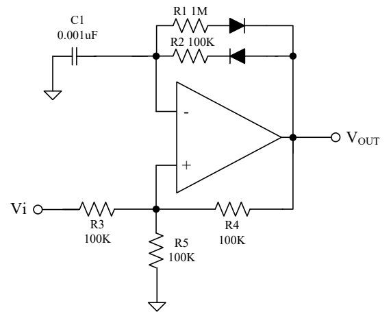
Pulse Generator
