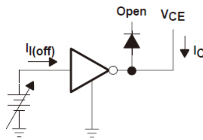
Figure 2. II(off) Test Circuit
