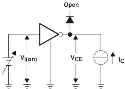
Figure 5. V_{I(on)} Test Circuit
